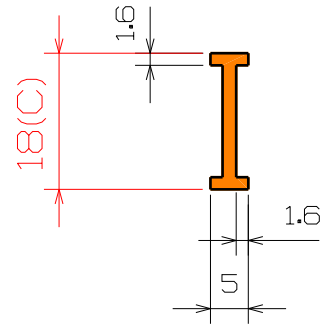
Section cut B-B
