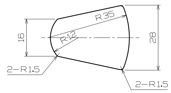
Section Cut B-B
