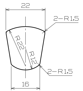
Section Cut C-C
