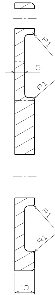
Section Cut A-A
